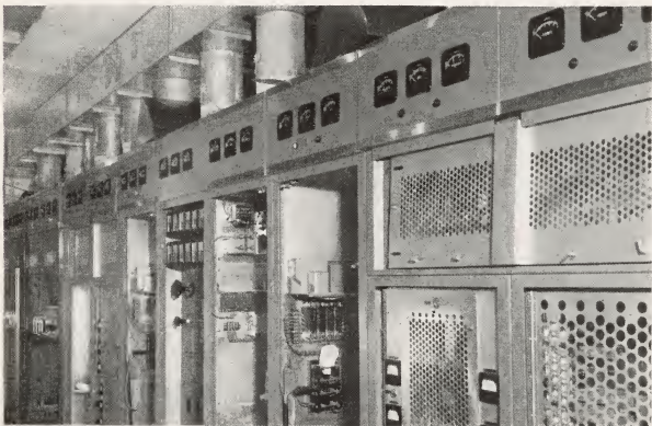
Five thousand watts of power from this giant RCA transmitter will enable WENR-TV to make its debut Sept. 17. Located on the 44th floor of the Civic Opera building, the unit is made up of eight cabinets, including sound and sight.
